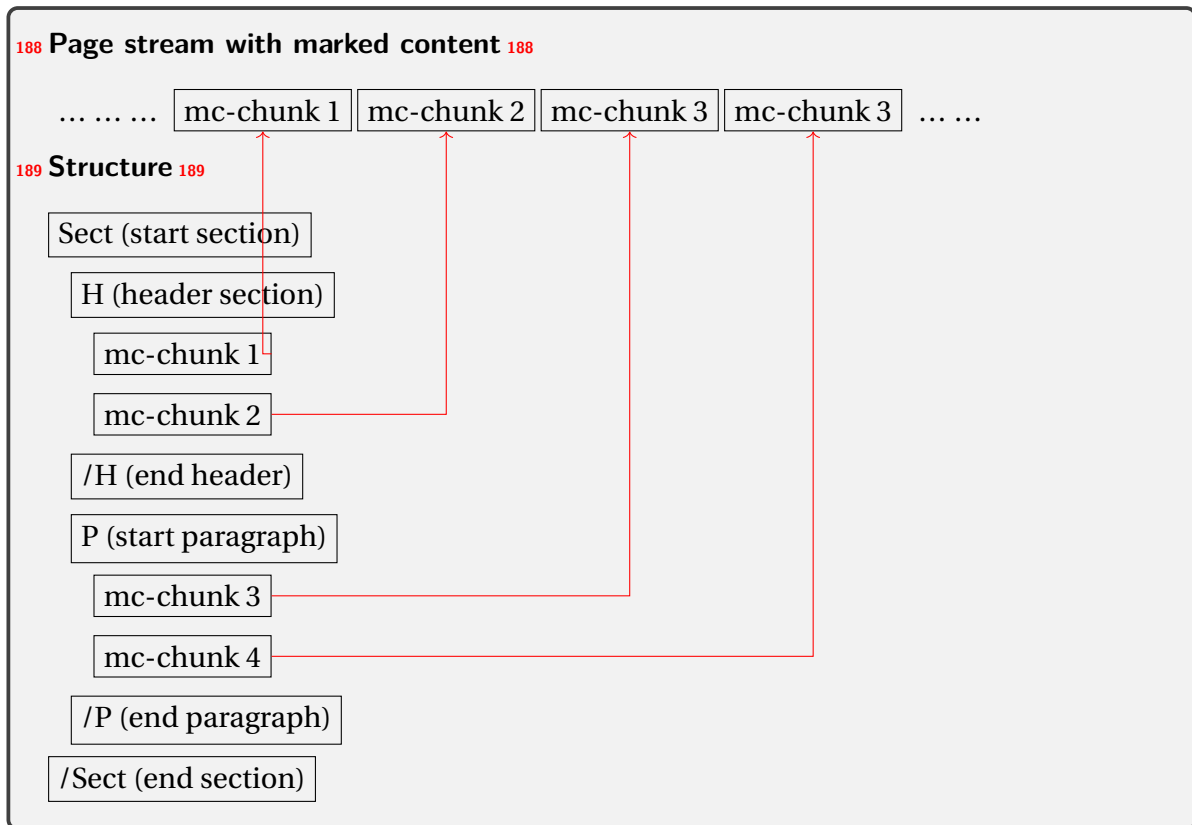
190 Figure 1: Schematical description of the relation between marked content in the page stream and the structure 190
